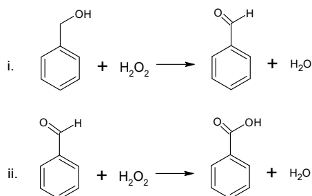
Fig.1. Sequential oxidation of benzyl alcohol to benzaldehyde and subsequent conversion to benzoic acid.
