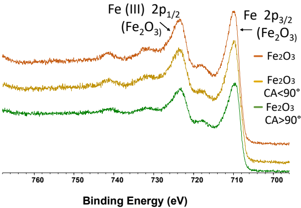
Fig. 9. High-resolution XPS spectra in the Fe 2p region for pristine and HDTMS-functionalized Fe 2 O 3 -NPs. Binding energies at 710 eV (Fe 2p 3/2 )
