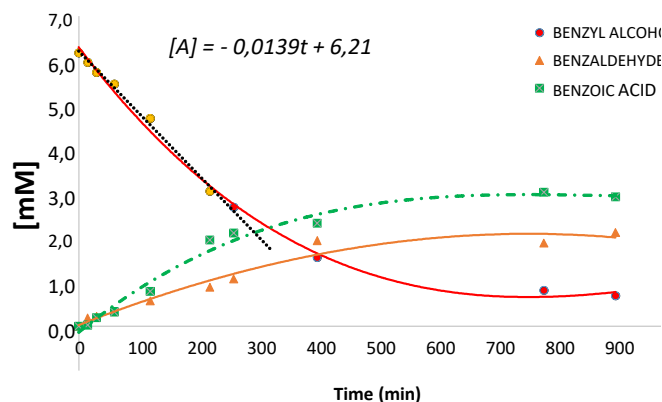
Fig. 5. Zero-order kinetic model for benzyl alcohol oxidation with \text{H}_2\text{O}_2 at 50^\circ\text{C} over superhydrophobic \text{Fe}_2\text{O}_3 -NPs (CA = 167^\circ , 40% HDTMS coverage) in Pickering emulsion. The linear regime ( [A] = -0.0139t + 6.21 ) is valid up to ~60% conversion; the kinetic transition at ~300 min indicates onset of consecutive oxidation reactions.
