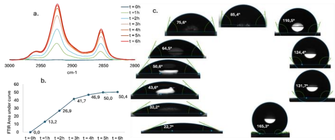
Fig. 7. Surface functionalization of Fe 2 O 3 -NPs with HDTMS. (a) DRIFT spectra in the C–H stretching region (2800–3000 cm -1 ) as a function of reaction time; (b) kinetics of HDTMS grafting monitored by the integrated C–H band intensity; (c) water contact angle as a function of HDTMS surface coverage (5–40%)
