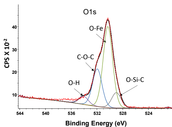
Fig. 11. High-resolution XPS spectra in the O 1s region for pristine and HDTMS-functionalized Fe _{2}O_3 -NPs.
