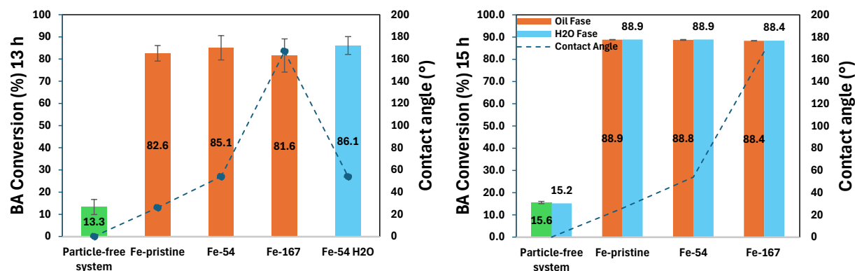
Fig. 4. Benzyl Alcohol Conversion in Oil and Aqueous Phases of Fe 2 O 3 -Stabilized Pickering Emulsions at Different Reaction Times.
