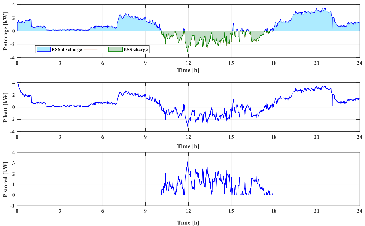
Fig. 5. Power in the HESS to match the load requirements (a), power in the HESS considering the long-term power components (b) and power delivered by the photovoltaic array to charge the HESS.
