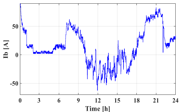
Fig. 7. Battery current.
