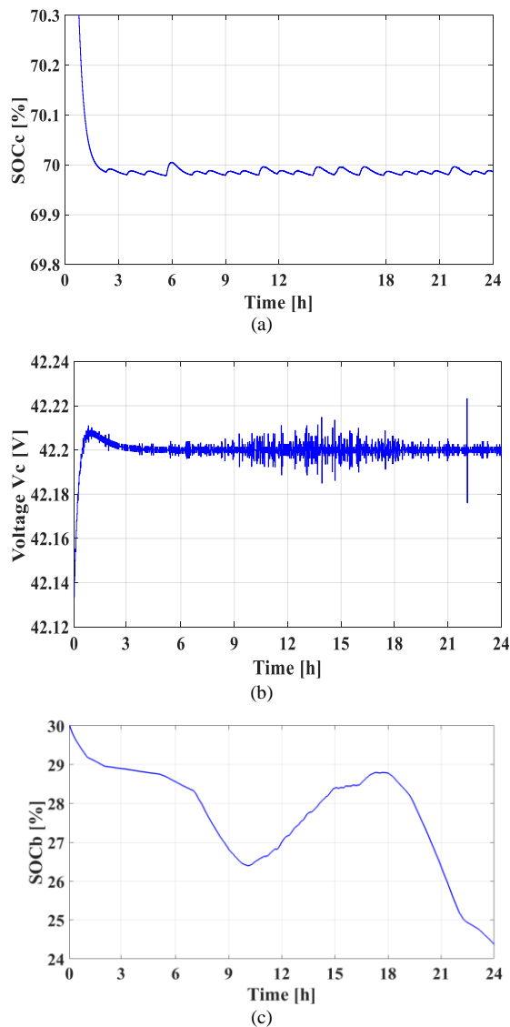
Fig. 6. SOC (a) and voltage (b) of the UCs, and batteries SOC (c).
