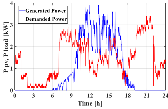
Fig. 3. Generation profile from the photovoltaic array (blue) and load profile (red).
