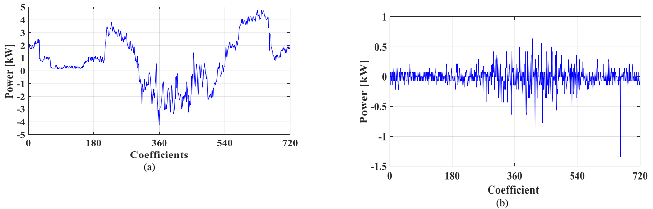
Fig. 4. Wavelet coefficients for low (a) and high frequencies (b).
