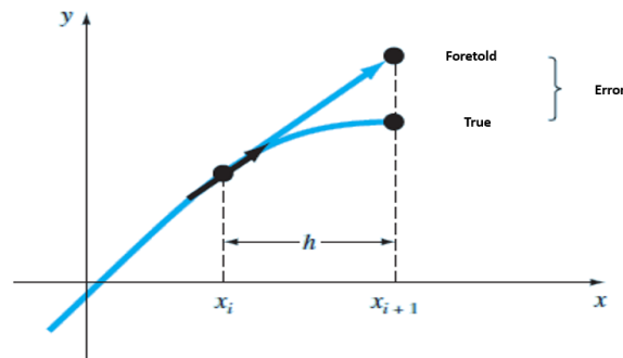
Fig. 2. Graphic demonstration of the Euler method. [3]
