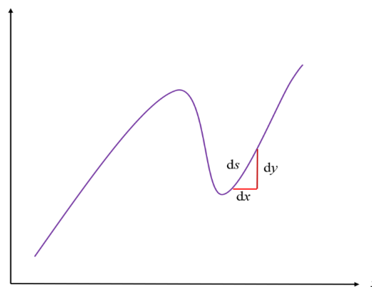
Fig. 1. The characteristic triangle. [1]
