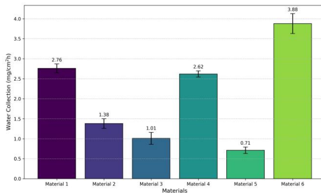
Fig. 13. Water capture testing of coated mesh materials in the laboratory.
