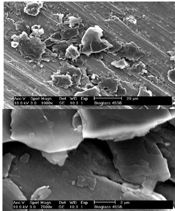
Figure 4. SEM pictures of bioglass powder.
